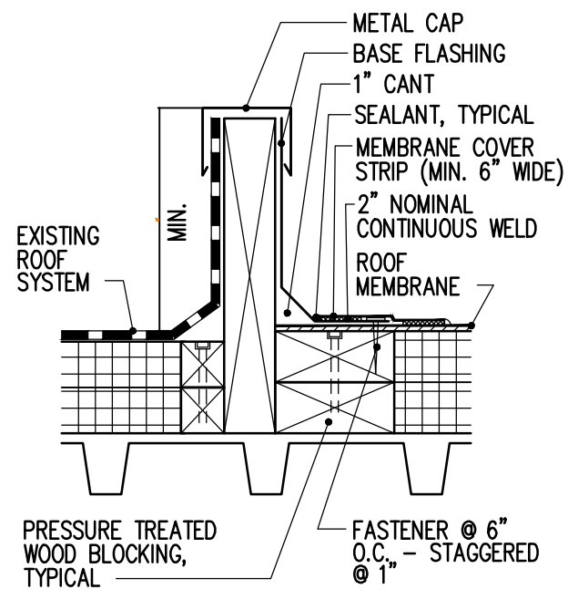
6 CURB DETAIL 3" = 1'-0"
