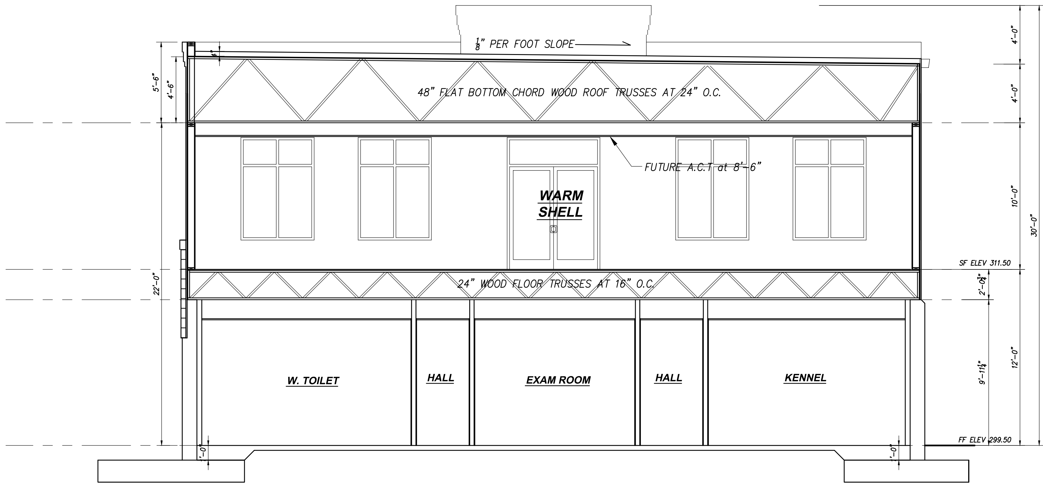
CROSS SECTION C SCALE: 1/4"=1'-0"
