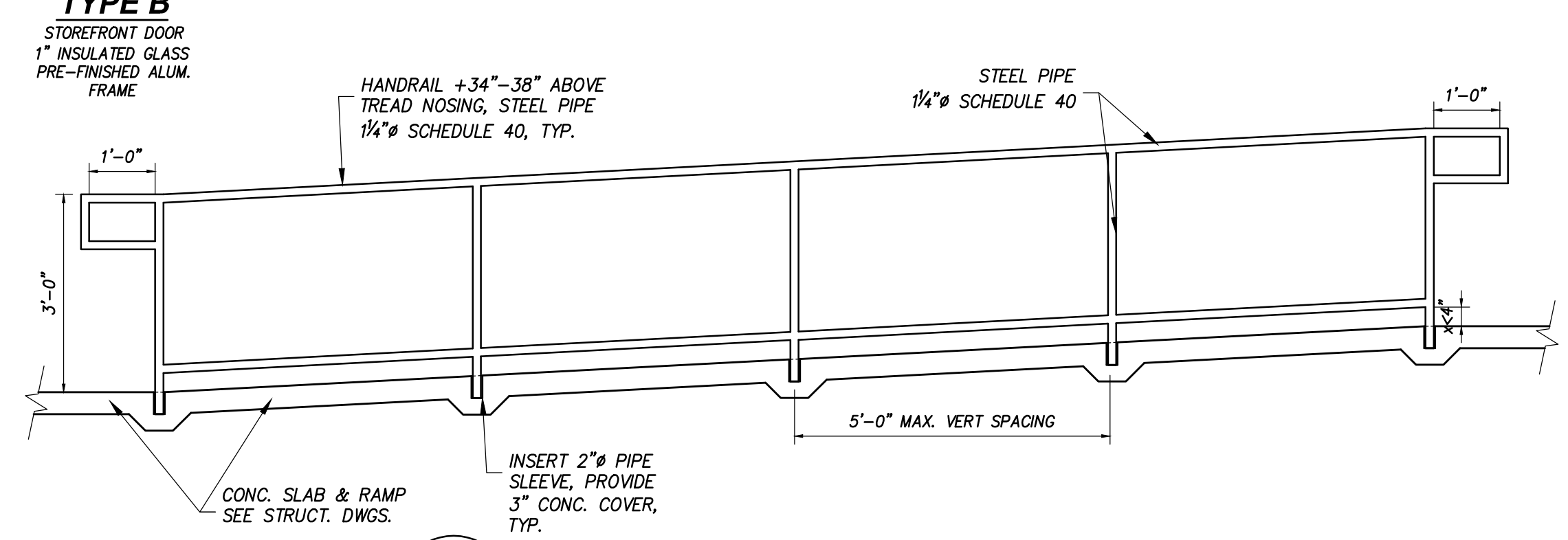
3 TYP. CONC. RAMP DETAIL A11
