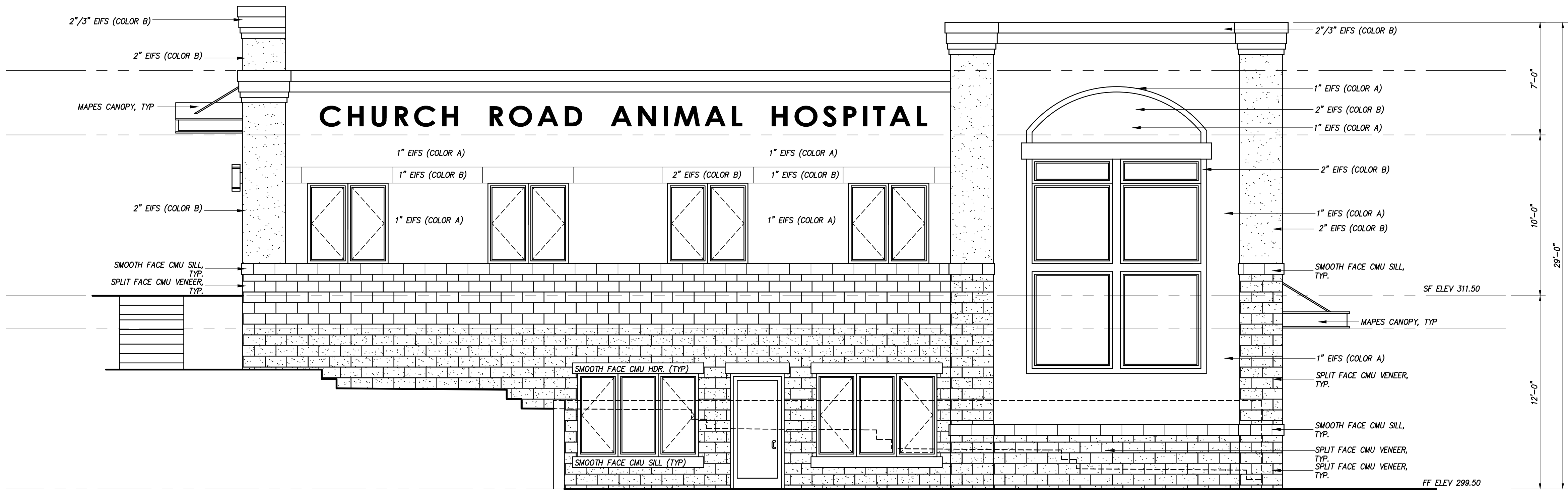
REAR ELEVATION
