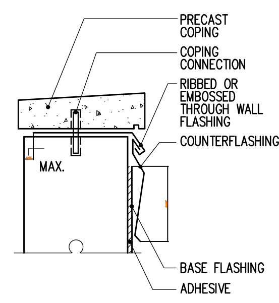
4 COPING DETAIL (ALTERNATE) 3" = 1'-0"
