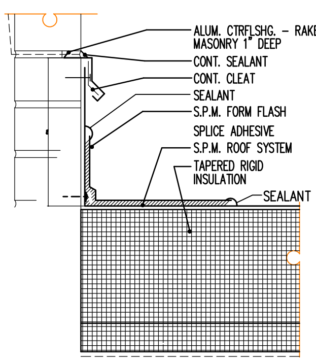
2 FLASHING DETAIL 3" = 1'-0"
