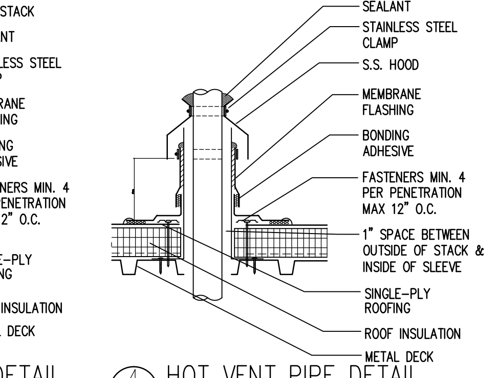
4 HOT VENT PIPE DETAIL 1 1/2" = 1'-0"
