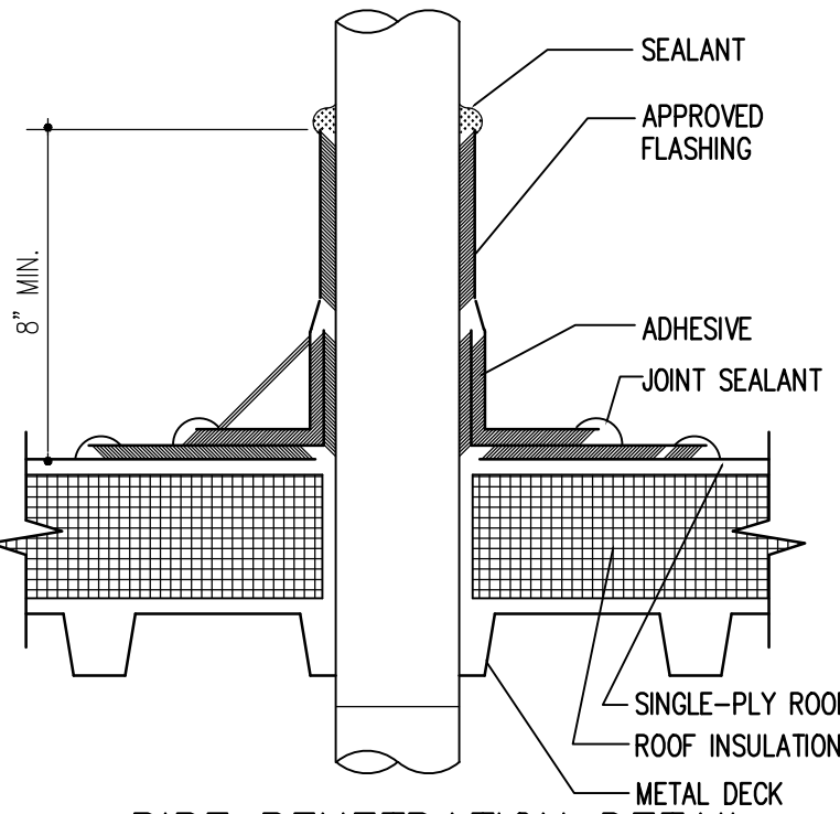
2 PIPE PENETRATION DETAIL 3" = 1'-0"
