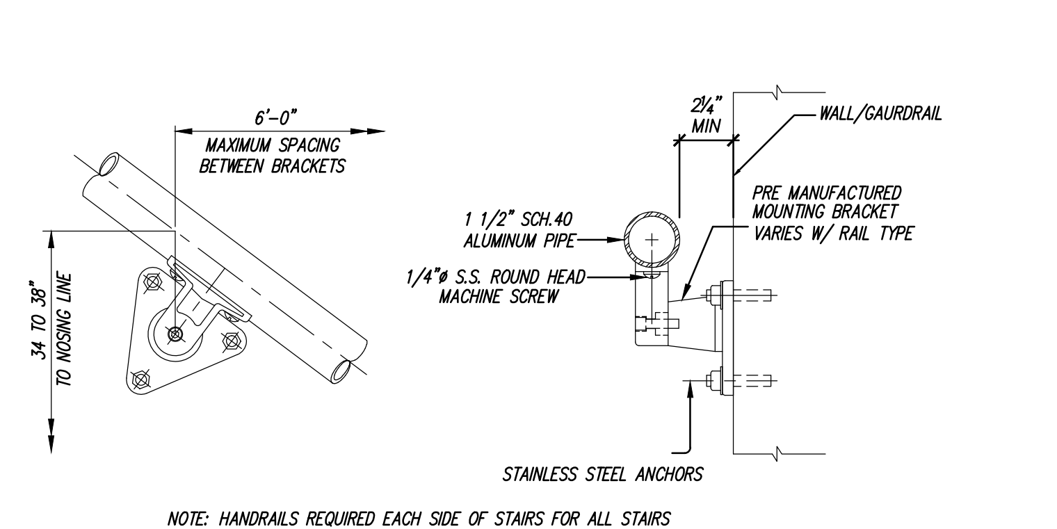
1 RAILING DETAIL A11 NOT TO SCALE
