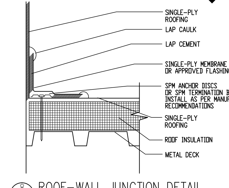
8 ROOF-WALL JUNCTION DETAIL 3" = 1'-0"
