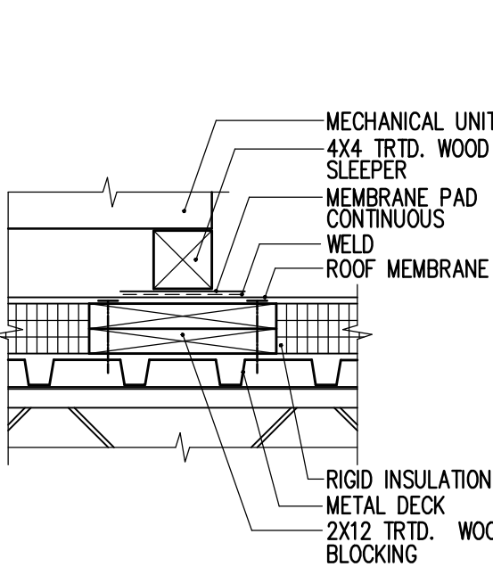
8 MECH. SUPPORT DETAIL 1 1/2" = 1'-0"
