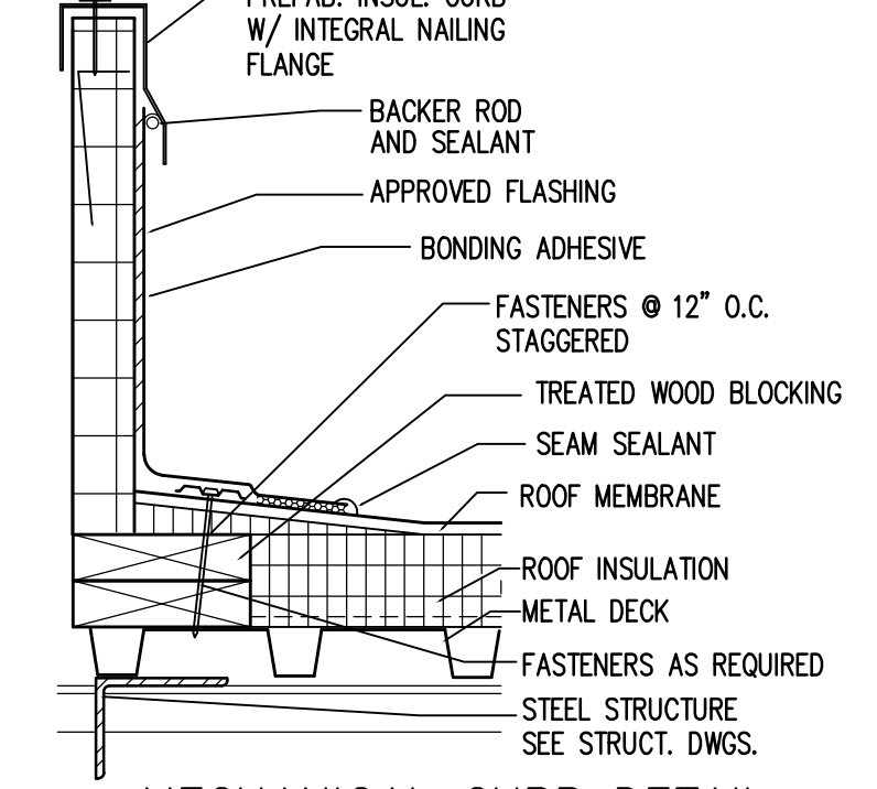
5 MECHANICAL CURB DETAIL 3" = 1'-0"
