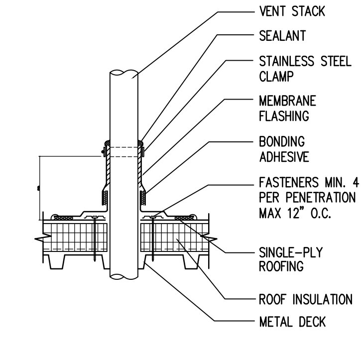
3 VENT PENETRATION DETAIL 1 1/2" = 1'-0"
