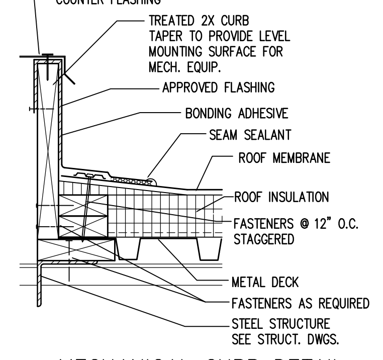
6 MECHANICAL CURB DETAIL 1 1/2" = 1'-0"
