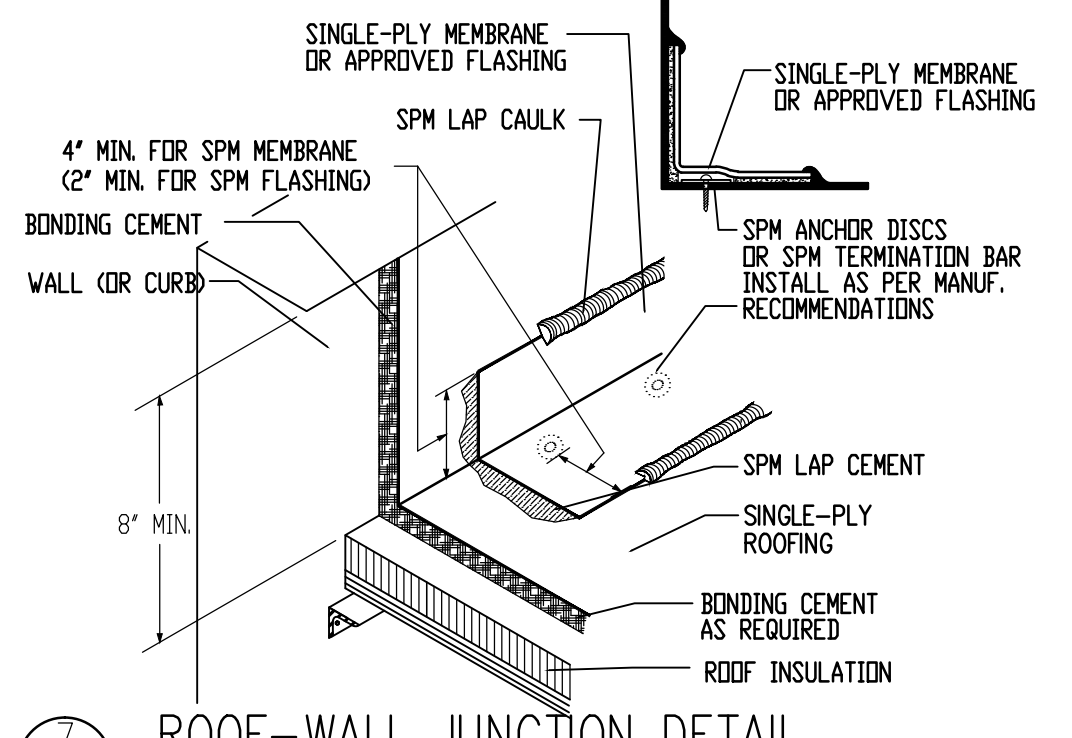
7 ROOF-WALL JUNCTION DETAIL N.T.S.
